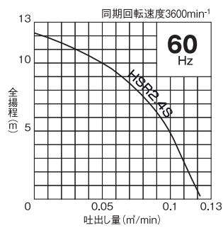
HSR2.4S
