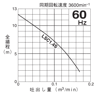
LSC-1.4S
