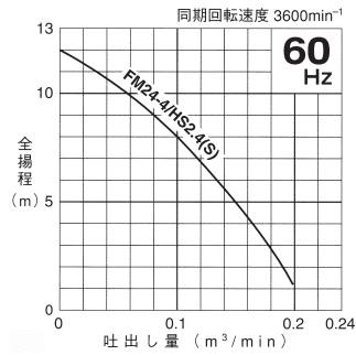
HS2.4S
